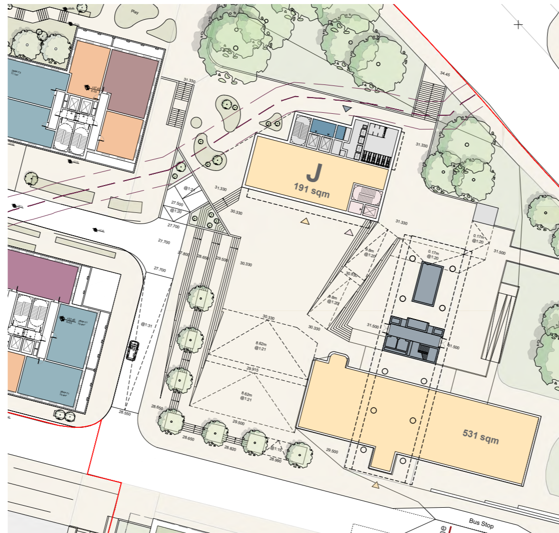
Floor Plan - Ground floor - Commercial areas shown yellow
